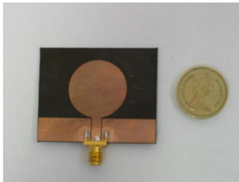
Fig. 1 1 Photograph of a monopole disk UWB antenna.
