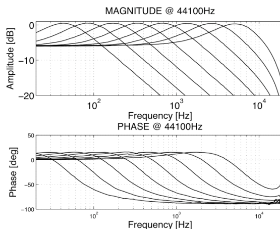
Figure 2: Magnitude vs. frequency and phase vs. frequency of the individual filters composing the decomposition filter for an 8-channel source mixture.
