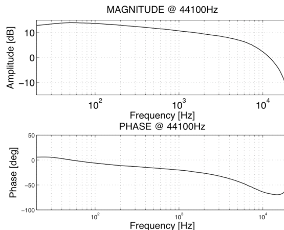
Figure 3: Magnitude vs. frequency and phase vs. frequency of the combined response of a derived decomposition filter for an 8 channel source mixture.
