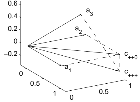
Fig. 3. Example of an external vertex ( c_{+++} ) in 3-D.
