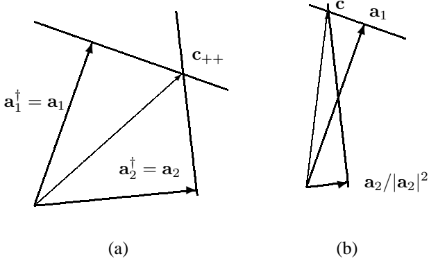
Fig. 2. Vertex c_{++} of unit basis set [+\mathbf{a}_1, +\mathbf{a}_2] , for (a) internal and (b) external vertex
