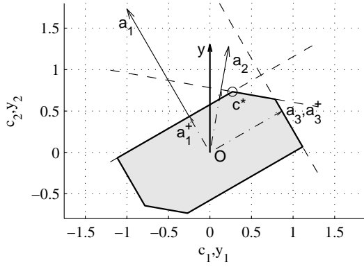
Fig. 1. Polytope P^* in 2-D with optimum basis vertex c^* .
