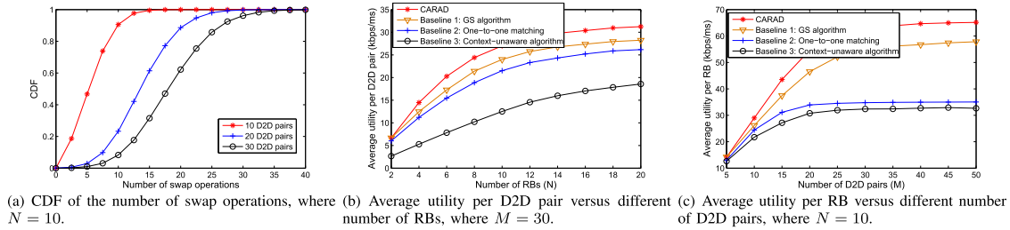
Fig. 1. Performance analysis of the proposed CARAD algorithm.
