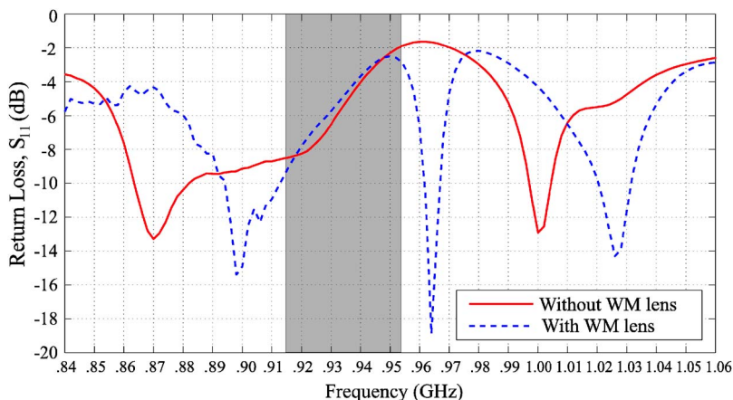
FIG. 3. (Color online) Return loss ( S_{11} parameter) as function of frequency for the meander-line antenna in the free space and at the interface of the wire medium slab.
