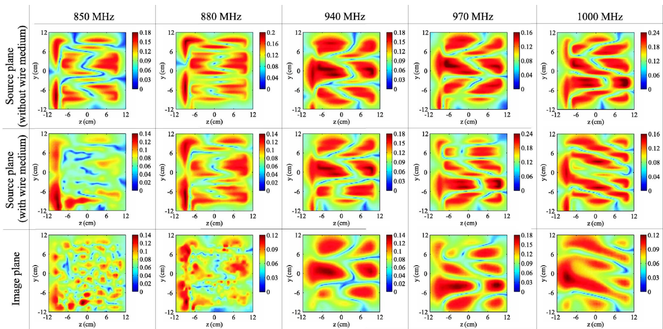
FIG. 2. (Color online) Results of the near field scan at 850 MHz, 880 MHz, 940 MHz, and 1 GHz (in arbitrary units): the amplitude of the component of electric field normal to the interface at 2 mm distance from the meander antenna in the free space (source plane without wire medium), the same but when the antenna is placed at the front interface of the transmission device (source plane with wire medium) and at 2 mm distance from the back interface of the wire medium slab (image plane).
