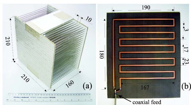
FIG. 1. (Color online) Geometries of the transmission device (a), a 21 \times 21 array of wires with 1 mm radii, and the near-field source (b). All dimensions are in millimeters.
