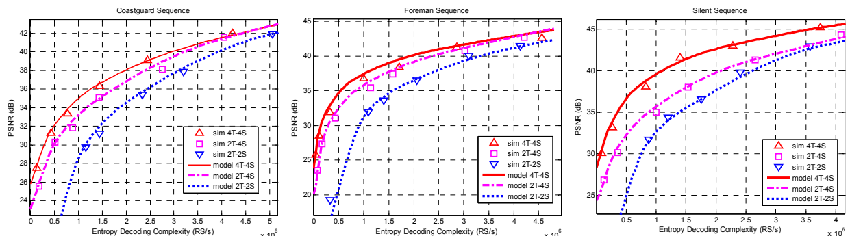
Figure 8. Entropy decoding complexity vs. distortion plots for different spatio-temporal decomposition parameters, where “S” and “T” indicate the number of spatial and temporal levels (respectively).
